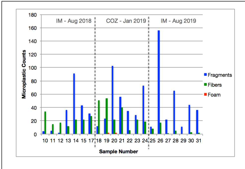
Figure 4: Total microplastic counts by particle type (fragment, fiber, and foam) Samples 10 through 17 and 25 through 31 were collected from the Reserva de la Biosfera Caribe Mexicano near Isla Mujeres (IM), while samples 18 through 24 were collected within the Parque Nacional Arrecifes de Cozumel off the western coast of Cozumel (COZ).
